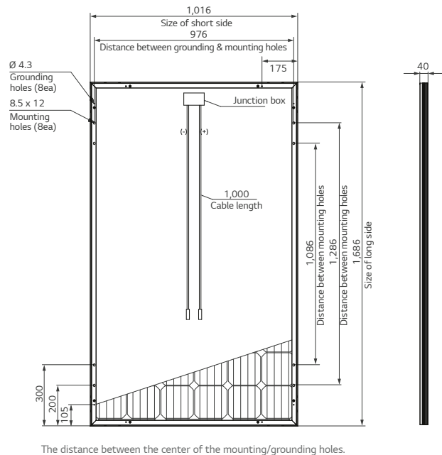
The distance between the center of the mounting/grounding holes.
